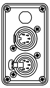
model PRE10-P TOP
