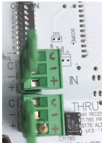
Control cable terminal block
